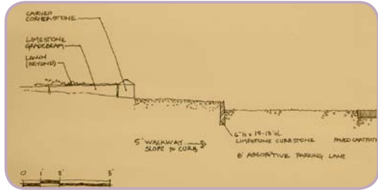
T4 - Crushed Stone - Typical Sidewalk Entry
